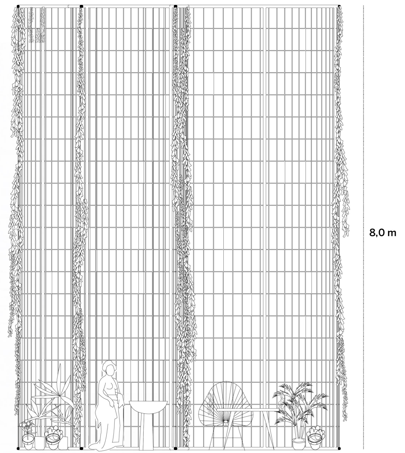
Section AA'
