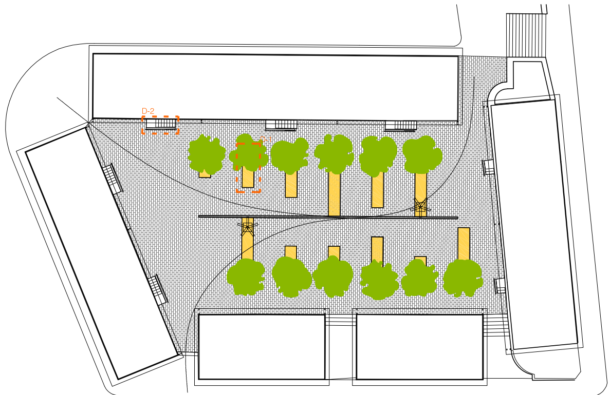
PLANTA, E: 1/400
