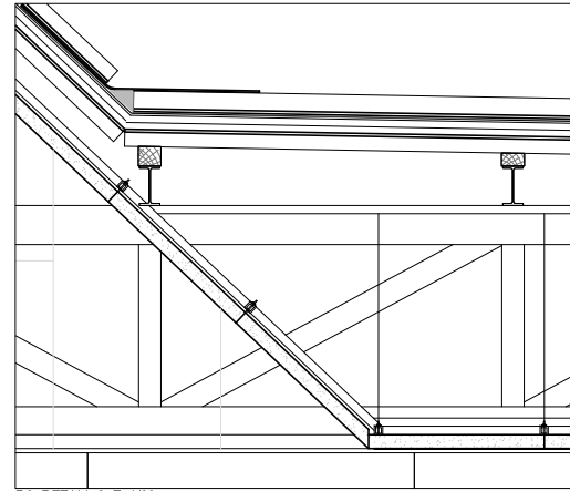
D3, DETALL 3, E: 1/30
