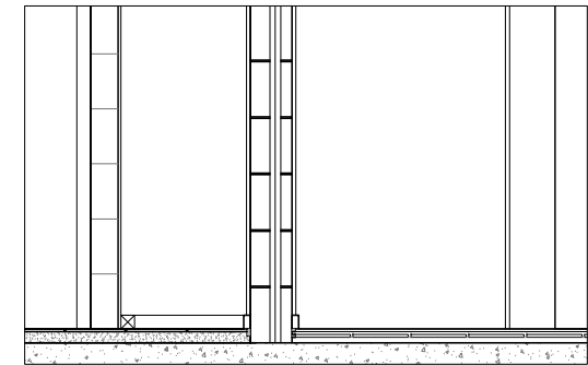
D8, DETALL 8, E: 1/30
