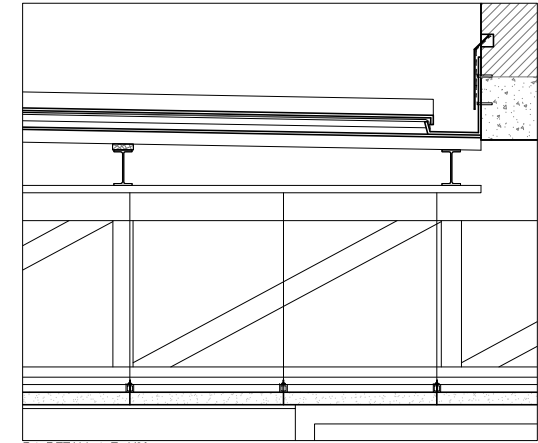
D4, DETALL 4, E: 1/30
