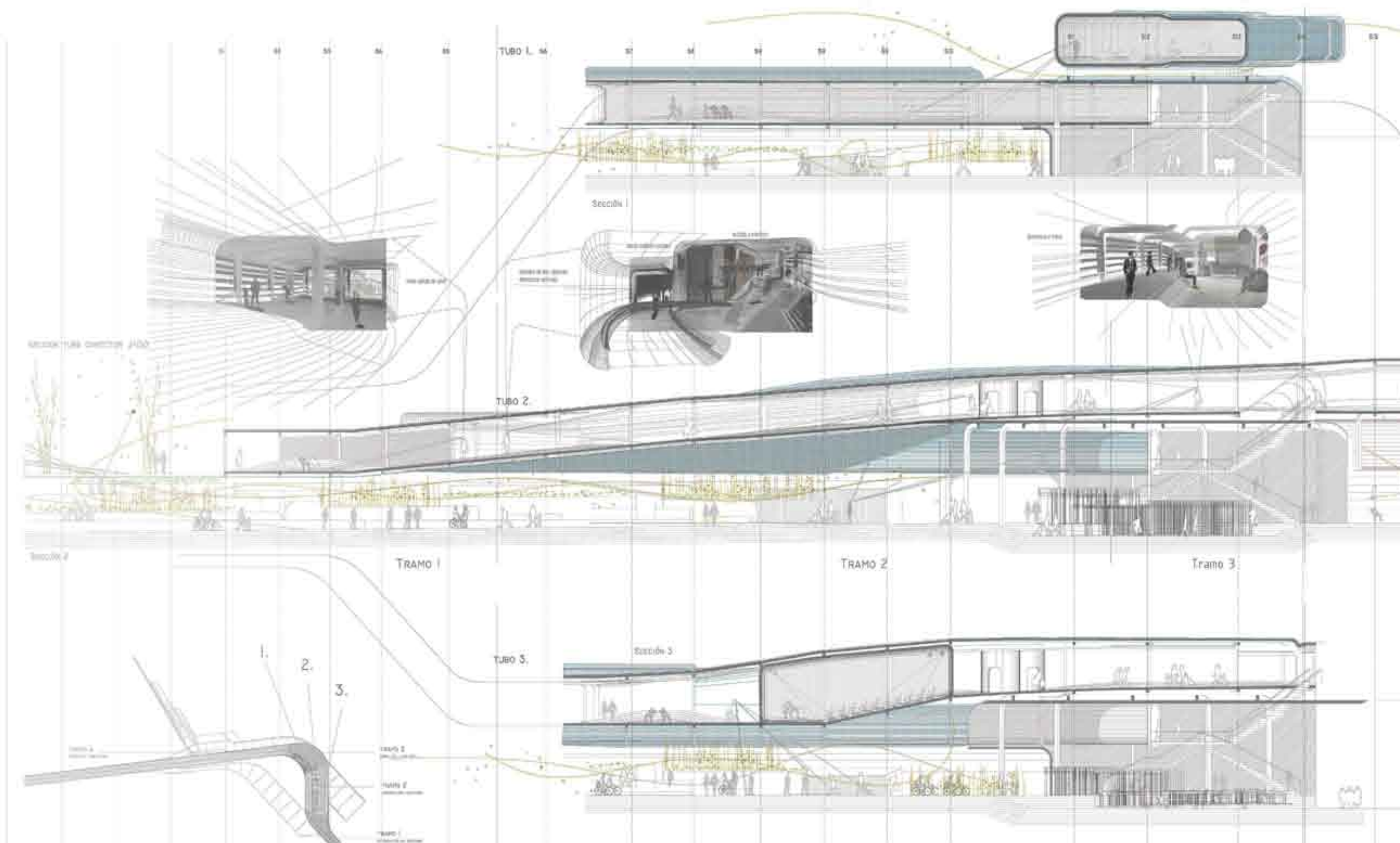
DEFORMED SECTIONS ALONG THE TUBE
